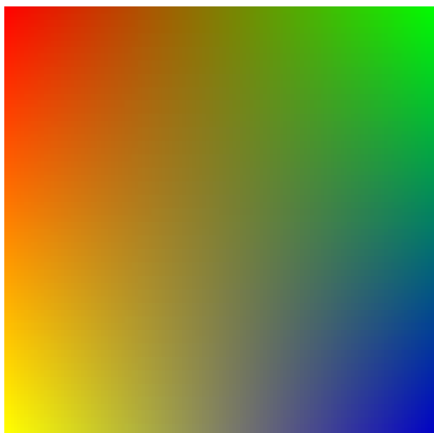
CoonsPatchMesh()
